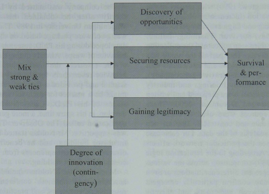
Figure 2. Research framework.
